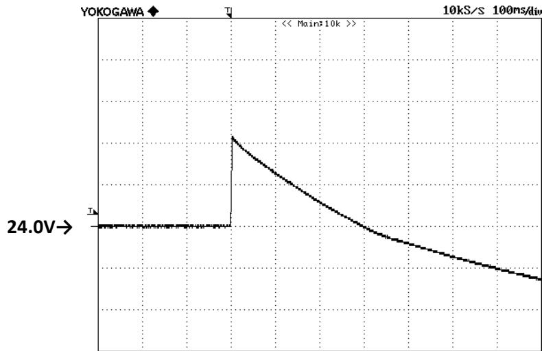
図16 過電圧波形 Fig.16 Over Voltage Waveform
