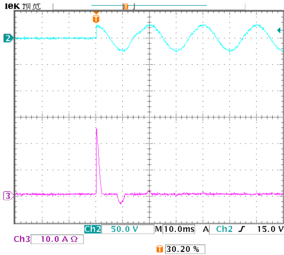
図15 突入電流波形 Fig.15 Inrush Current Waveform
