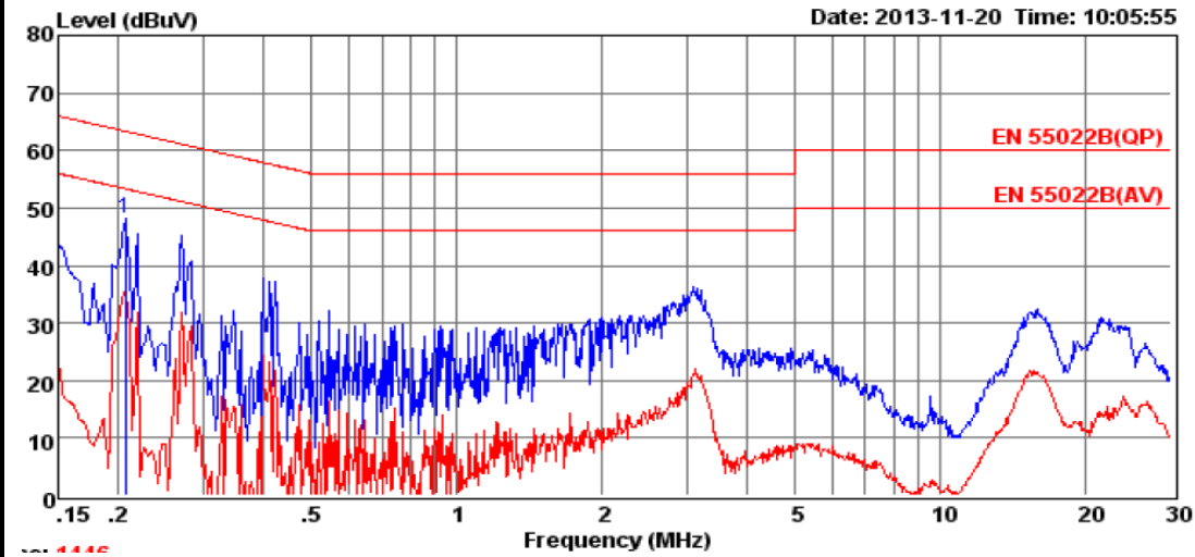
図18 雑音端子電圧 Fig.18 Conduction Noise Waveform
