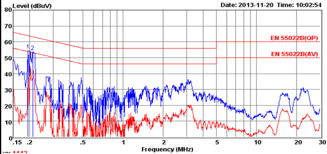
図18 雑音端子電圧 Fig.18 Conduction Noise Waveform
