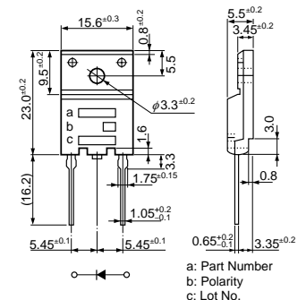
• No. 21 TO-3PF2Pin
