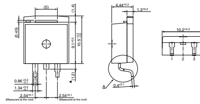
• No. 5 Surface-Mount (TO220S)
